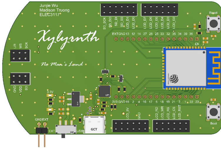
Realistic View Front
